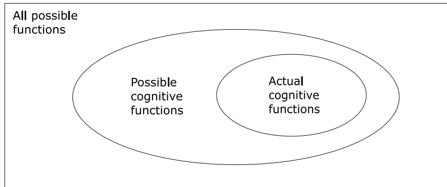
Figure 1: The set of functions describing actual cognitive capacities is a subset of the set of functions describing possible cognitive capacities.
