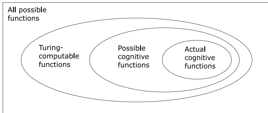
Figure 2: On the Church-Turing thesis, the set of functions describing possible cognitive capacities is a subset of the class of Turing-computable functions.
