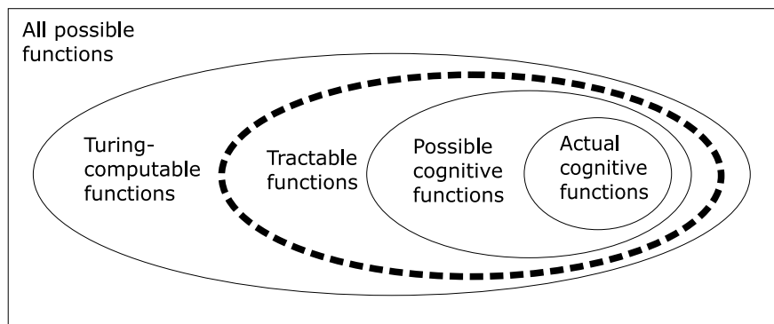
Figure 3: According to the Tractable Cognition thesis the set of functions describing possible cognitive capacities is a subset of the set of tractable functions. The dotted line indicates that the set of tractable functions remains to be formalized.
