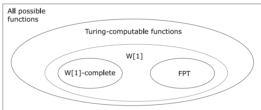
Figure 9: The view of W[1] on the assumption that FPT \neq W[1] . W[1] -complete parameterized problems are not in FPT if and only if FPT \neq W[1] .
