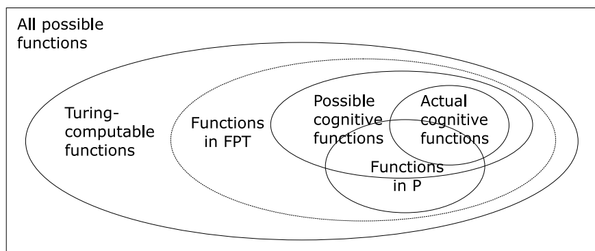
Figure 7: According to the FPT-Cognition thesis the set of functions describing possible cognitive capacities is a subset of the set of functions that are fixed-parameter tractable (FPT) for small parameters. The set FPT includes the functions in P as special cases.
