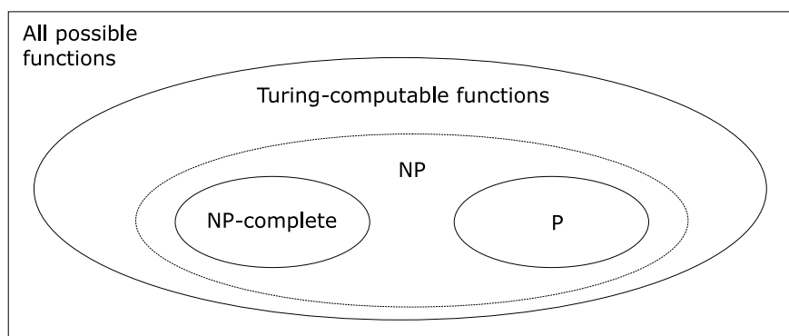
Figure 5: The view of NP on the assumption that P \neq NP . NP-complete problems are not in P if and only if P \neq NP .
