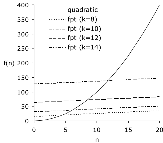
Figure 11: The figure compares quadratic polynomial-time O(n^2) with fpt-time O(\sqrt{2}^k + n) for parameter k = 8, 10, 12 , and 14 . Increasing the value of k causes the curve for fpt-time to translate upwards.
