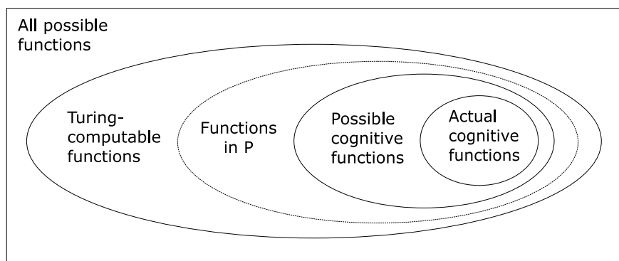
Figure 4: According to the P-Cognition thesis the set of functions describing possible cognitive capacities is a subset of the set of polynomial-time computable functions, P.
