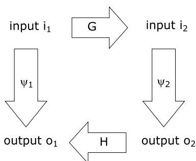
Figure 6: Illustration of the concept of polynomial-time reduction: The functions G and H together constitute a reduction from \psi_1 to \psi_2 if and only if \psi_1(i_1) = H(\psi_2(G(i_1))) . In that case the function \psi_1(i_1) can be computed by first computing i_2 = G(i_1) , then computing o_2 = \psi_2(i_2) , and finally computing H(o_2) = \psi_1(i_1) . The reduction is a polynomial-time reduction if and only if G and H are polynomial-time computable. In that case \psi_1 is polynomial-time computable if \psi_2 is polynomial-time computable.
