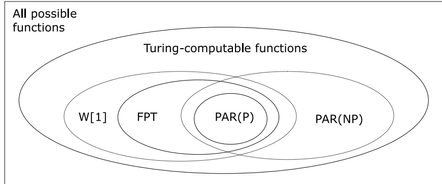
Figure 10: Illustration of the relationship between classes W[1] , FPT, P and NP. Because W[1] and FPT are classes of parameterized problems we cannot compare them directly to the classes P and NP. Therefore we define the class of all possible parameterizations of problems in P, denoted PAR(P) , and the class of all possible parameterizations of problems in NP, denoted PAR(NP) . Since P \subseteq NP , we have PAR(P) \subseteq PAR(NP) . Further, since every problem in P is in FPT for any parameter we have PAR(P) \subseteq FPT \subseteq W[1] .
