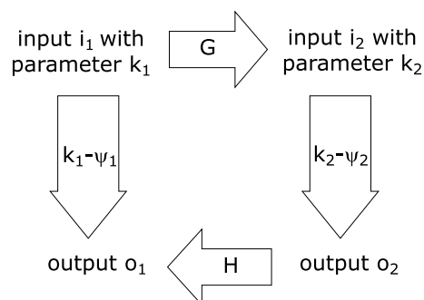
Figure 8: Illustration of the concept of parametric reduction: The functions G and H together constitute a parametric reduction from k_1\text{-}\psi_1 to k_2\text{-}\psi_2 if and only if \psi_1(i_1) = H(\psi_2(G(i_1))) such that k_2 = f(k_1) and both functions G and H are computable in fpt-time. In this case \psi_1 is fixed-parameter tractable for parameter k_1 if \psi_2 is fixed-parameter tractable for parameter k_2 .
